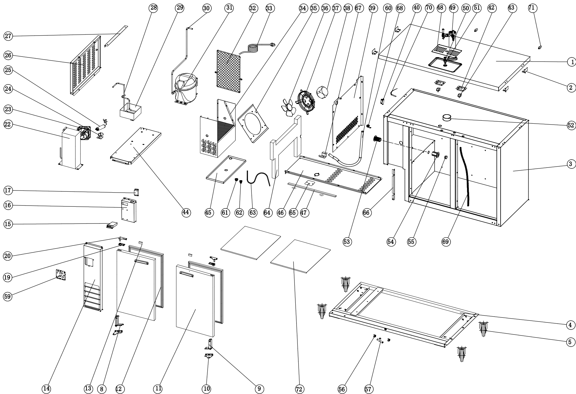
EXPLODE DRAWING OF BCBD48-1
