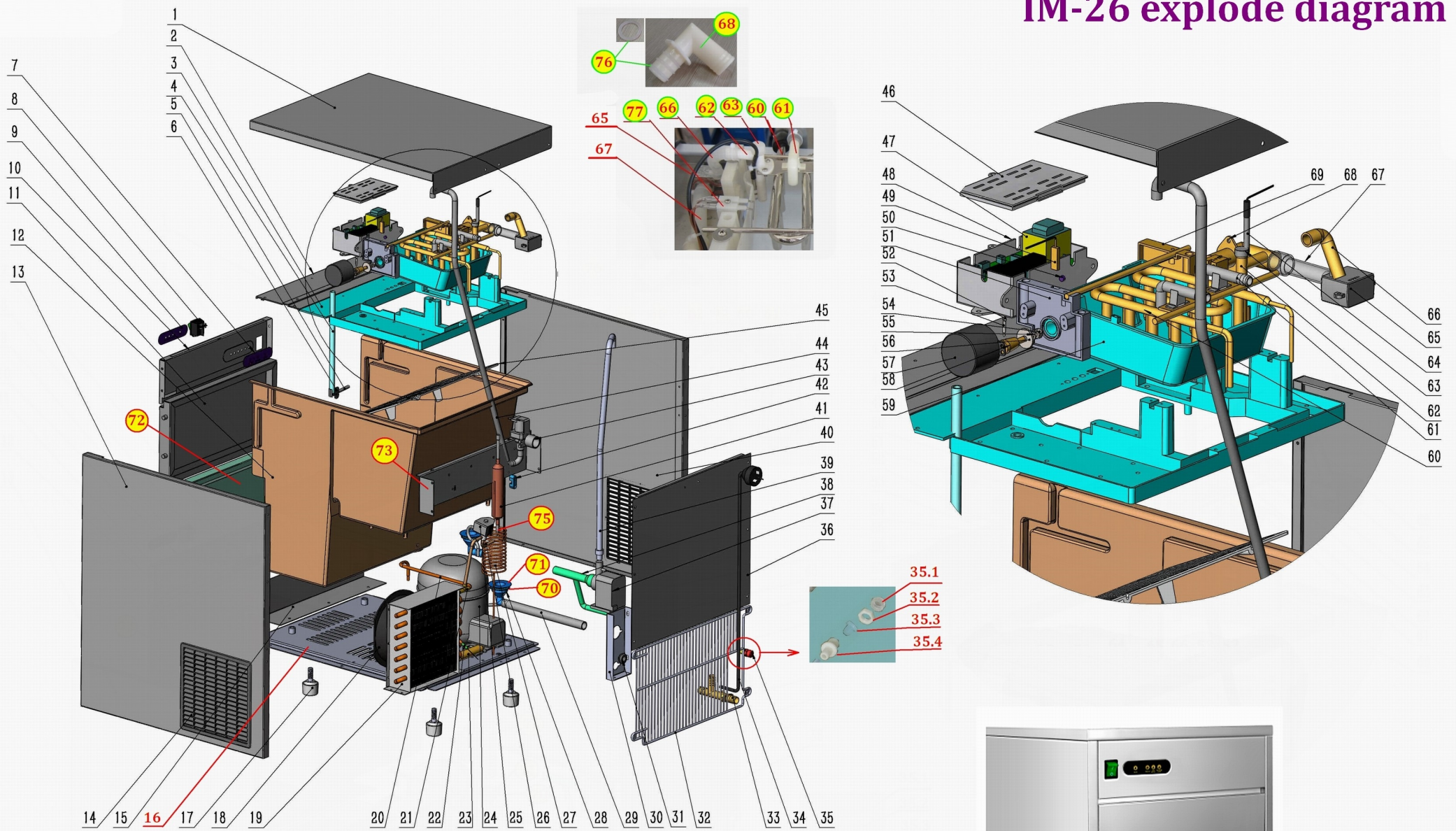
components list of IM-26 explode diagram
