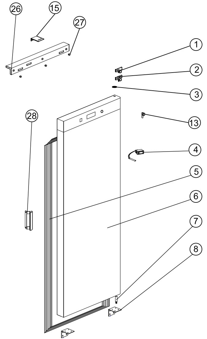
EXPLODE OF G-HT400F SS
