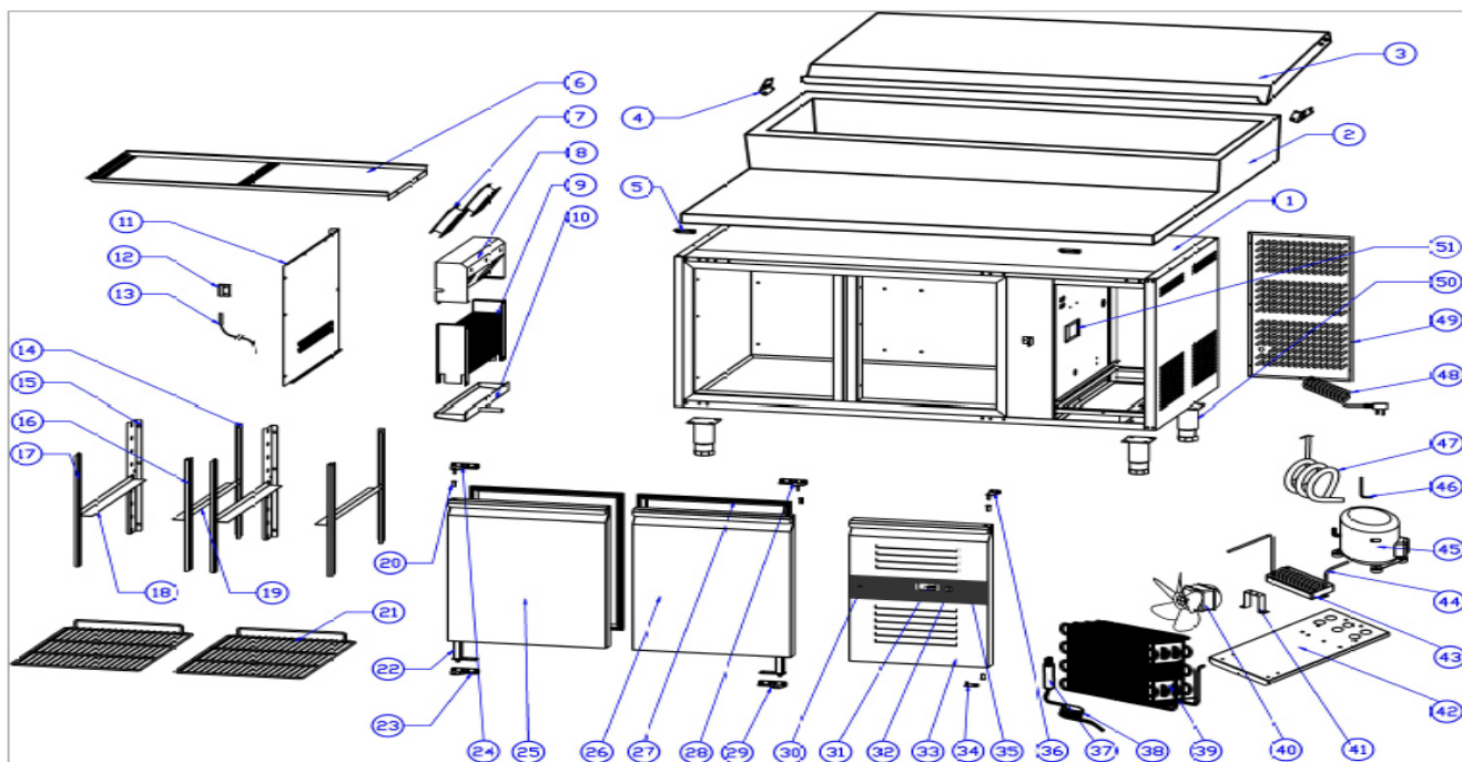
EXPLODED VIEW OF SH2800/SH2700
